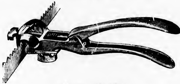
FOR HAND AND TENON SAWS
